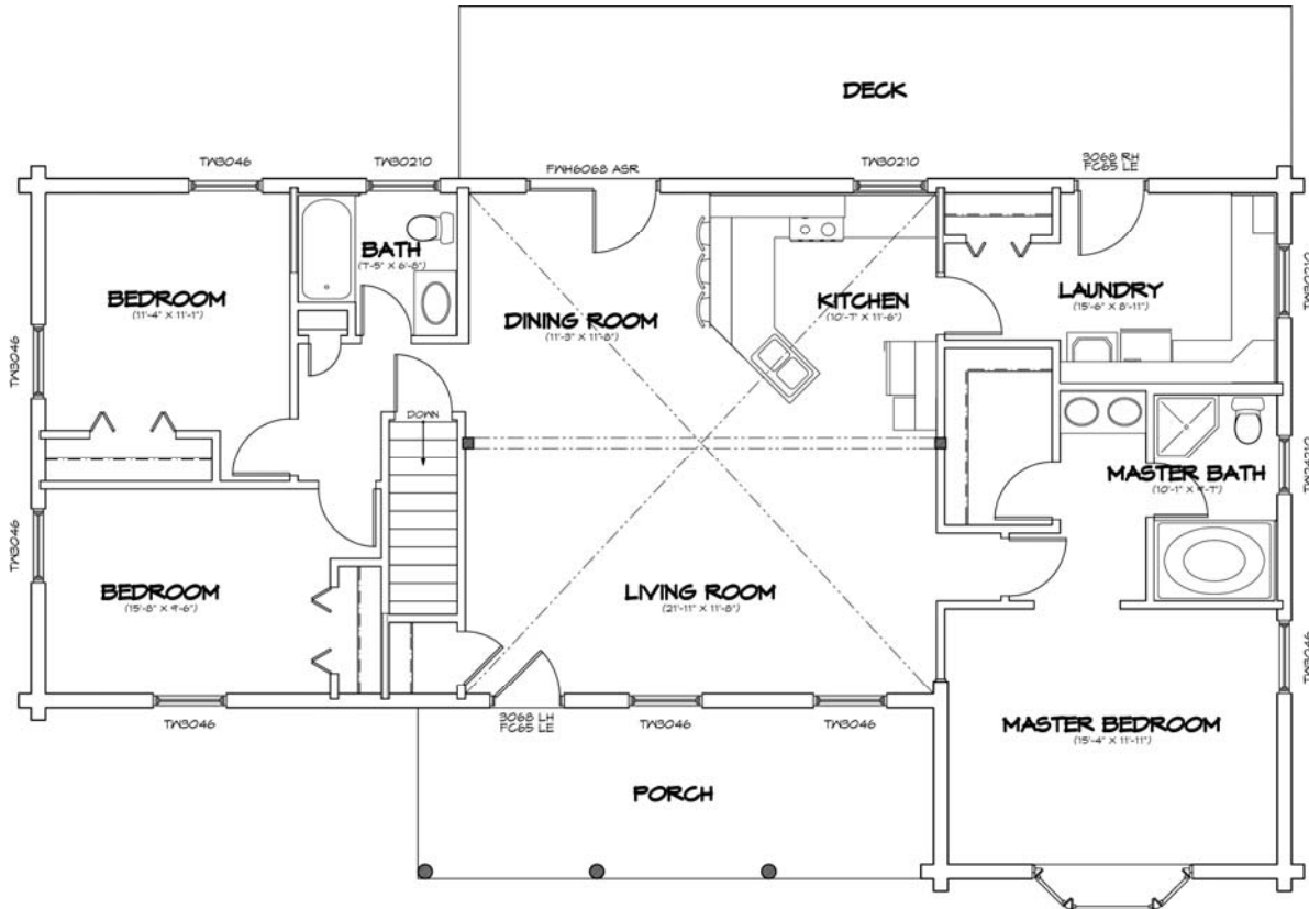
FLOOR PLAN
